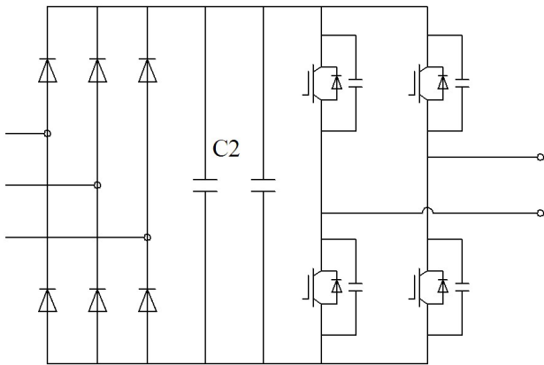
Typical circuit
