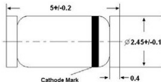
Glass Case MELF Dimensions in mm
