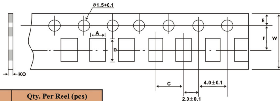
Tape and Reel Dimensions Unit : mm
