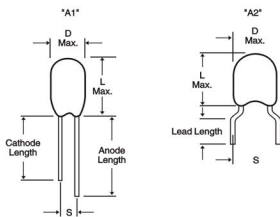
Sintered Cylindrical Epoxy-coated Solid Electrolyte Tantalum Capacitor
